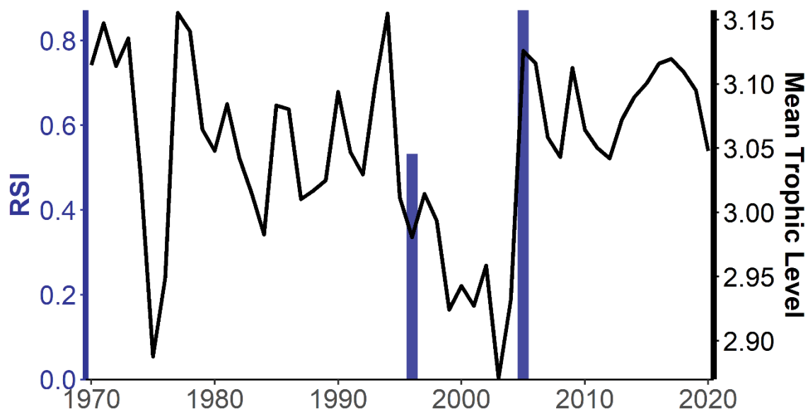
Figure 3. Abrupt shifts in the mean trophic level (MTL) identified using Rodionov's Regime Shift Index (RSI) method. The black line represents the MTL trend, while the blue bars indicate RSI scores.
