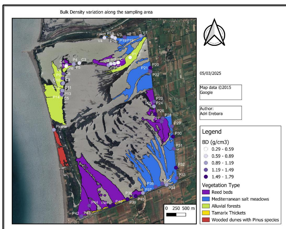
Figure 18. Bulk Density variation in Kune Vaini Lagoon (map data: Google Earth, QGIS, 3.34.7-Prizren)
