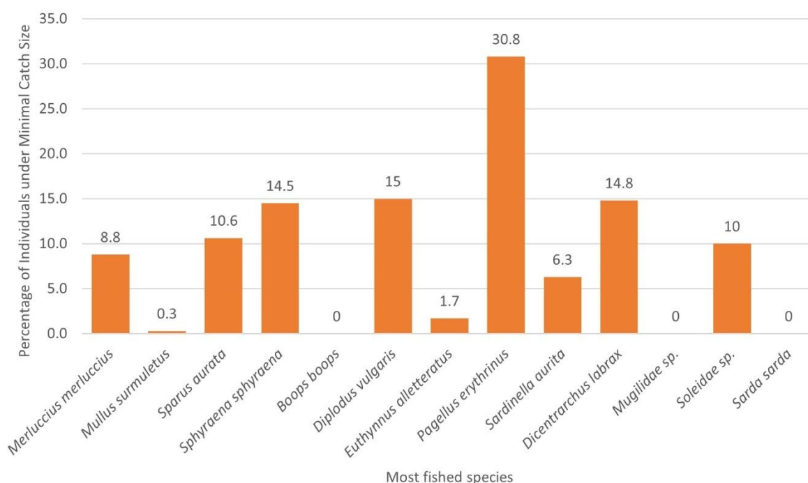
Figure 5. Graphical presentation of the percentage of fish individuals under the minimal catch size for each of the most fished species, which were fished by the small-scale fishers during the conducted study.
