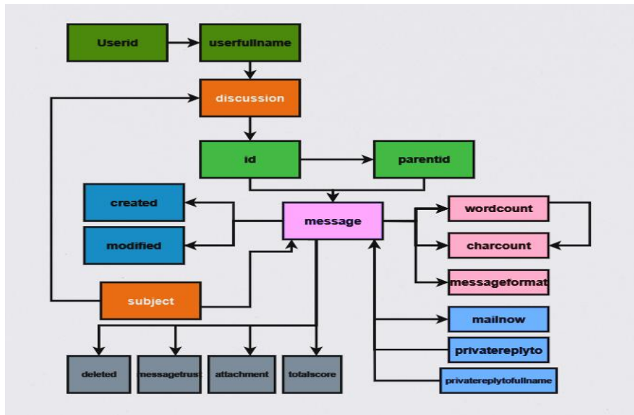
Figure 1. The structure of the raw log data from the Moodle platform. (source: own presentation)
