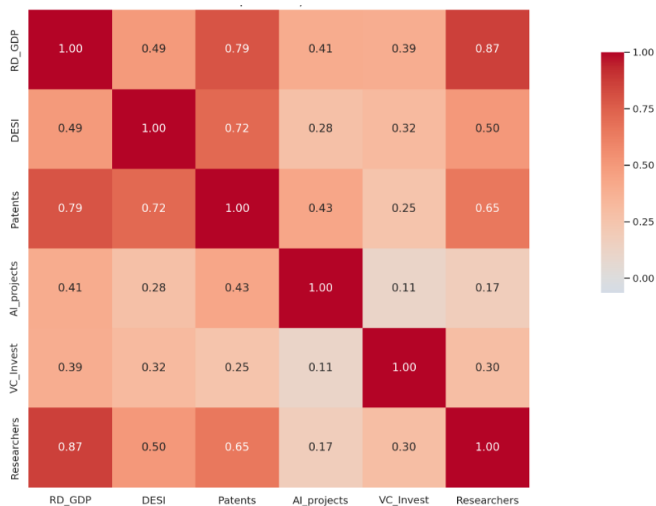
Figure 6. Correlation outputs_heatmap_2022, Reference: authors' elaboration.
