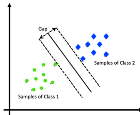
Figure 7: Support Vector Machine
