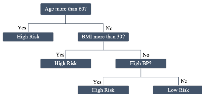
Figure 6: Decision Tree (Heart Attack Risk)
