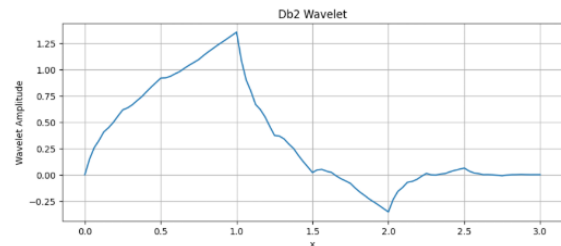
Figure 1: Daubechies Wavelets
