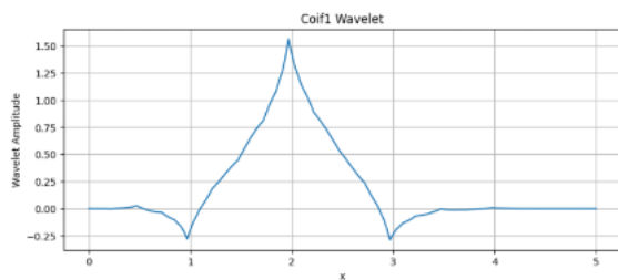
Figure 2: Coiflet Wavelets
