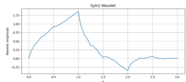
Figure 3: Symlet Wavelets
