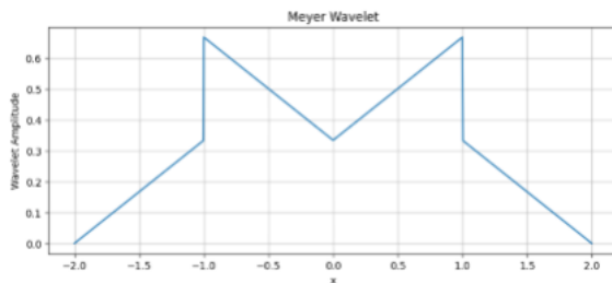
Figure 5: Meyer Wavelets
