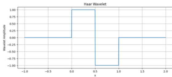
Figure 4: Haar Wavelets
